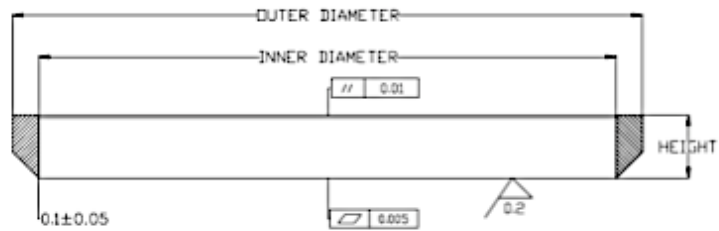
SS TYPE(SINGLE BLADE, SINGLE BEVEL TYPE)
