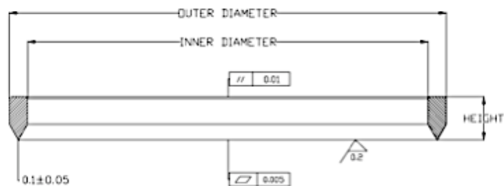
SD TYPE(SINGLE BLADE, DOUBLE BEVEL TYPE)
