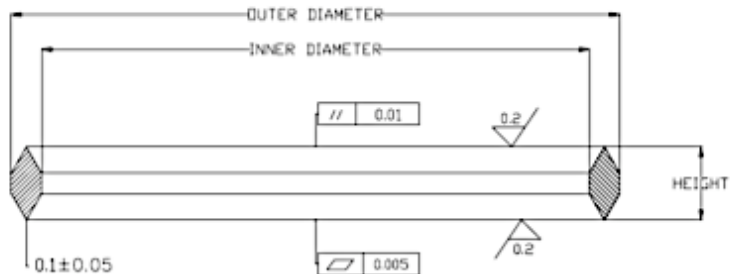
DD TYPE(DOUBLE BLADE, DOUBLE BEVEL TYPE)
